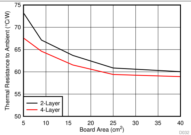
图 8. Package Thermal Resistance vs Board Copper Area, No Air Flow
