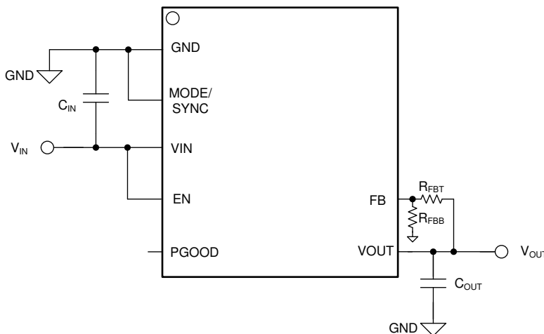
图 37. Adjustable 1.2-V to 15-V Output Typical Application Circuit
