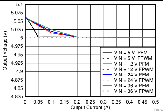
图 77. Line and Load Regulation for V_{OUT} = 5\text{ V}
