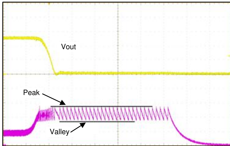
图 32. Current Limit Operation During Output Short Circuit
