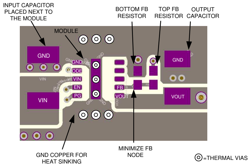
图 83. Layout Example With Adjustable Output Version
