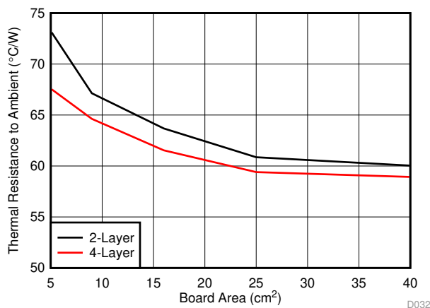
图 81. Package Thermal Resistance vs Board Copper Area
