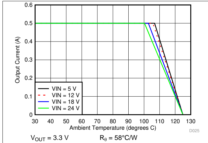
图 19. Ambient Temperature vs Output Current
