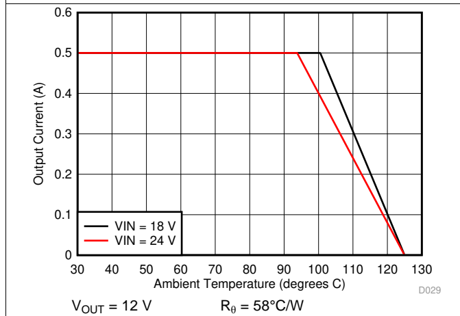
图 21. Ambient Temperature vs Output Current
