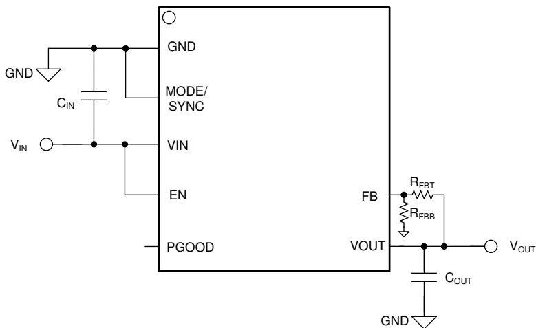
图 35. Adjustable 1.2-V to 15-V Output Typical Application Circuit
