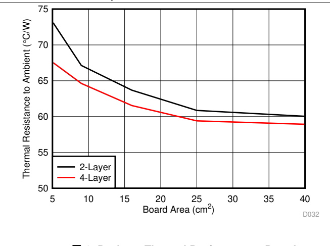
图 8. Package Thermal Resistance vs Board Copper Area, No Air Flow
