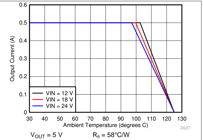
图 20. Ambient Temperature vs Output Current
