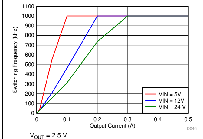
图 23. Auto PFM Mode Switching Frequency vs Output Current
