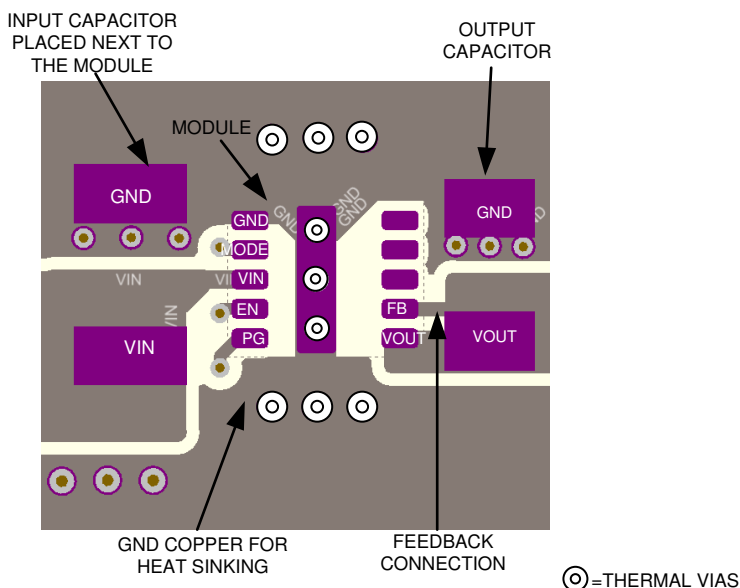
图 82. Layout Example With Fixed Output Version
