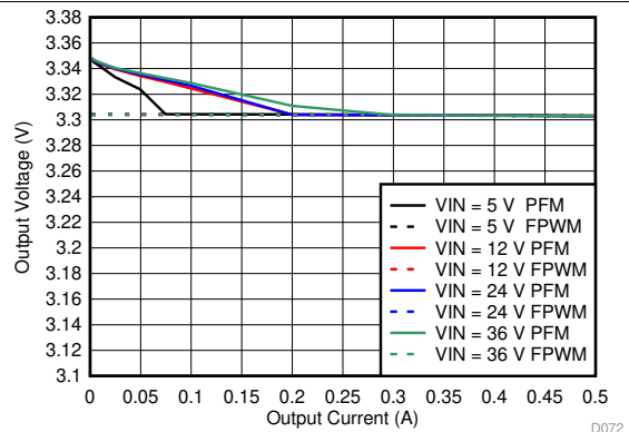
图 78. Line and Load Regulation for V_{OUT} = 3.3\text{ V}
