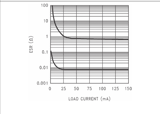
图 6-36. 2.2-µF Stable ESR Range for Output Voltage ≤ 2.3 V for Legacy Chip
