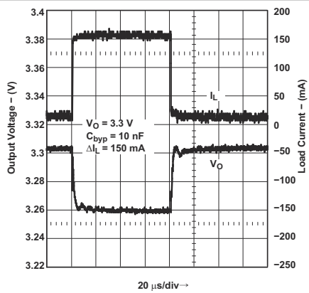
图 8-5. Load Transient Response for Legacy Chip
