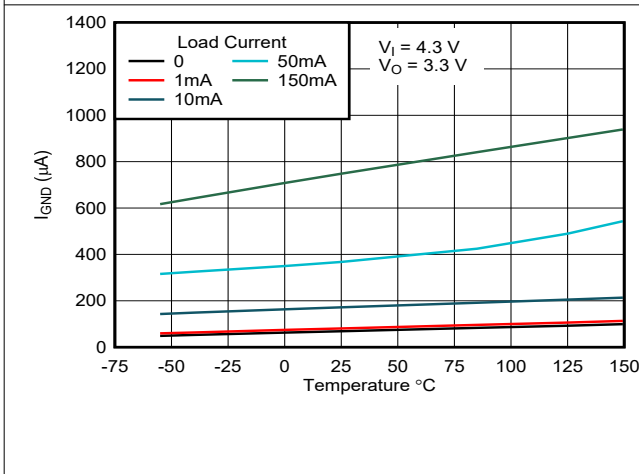
图 6-35. Ground-Pin Current vs Temperature for New Chip
