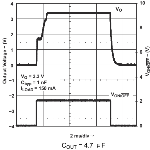
图 8-21. Turn-On Time for Legacy Chip
