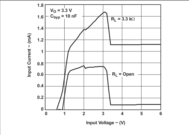
图 6-32. Input Current vs Input Voltage for Legacy Chip
