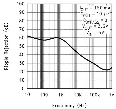
Figure 8. Ripple Rejection
