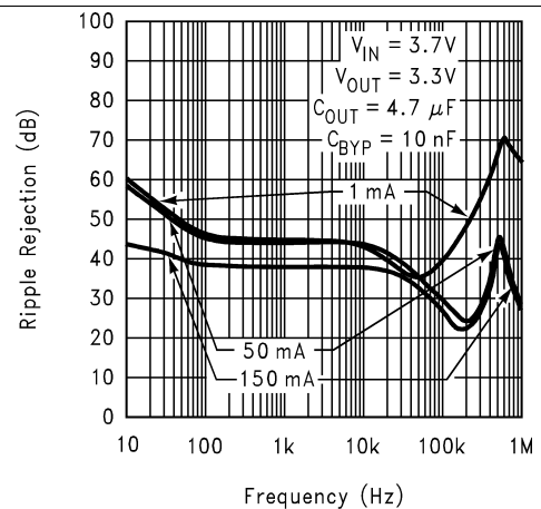
Figure 12. Ripple Rejection
