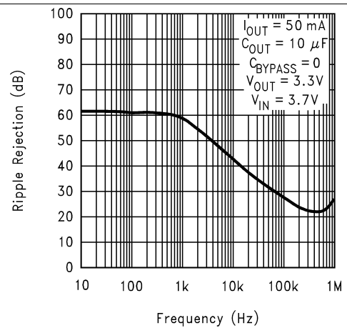
Figure 10. Ripple Rejection
