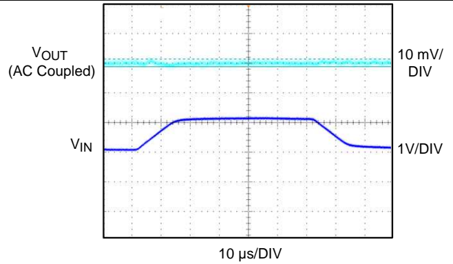
Figure 8. Line Regulation
