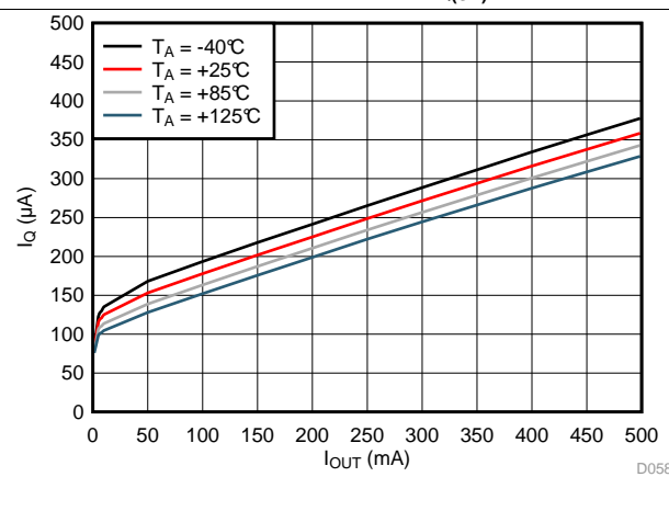
Figure 18. LP5912-1.8 I_{GND} vs I_{OUT}
