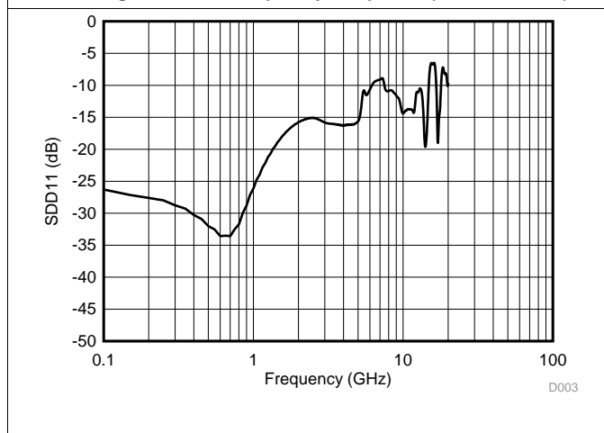
Figure 25. RX Differential Input Return Gain vs Frequency
