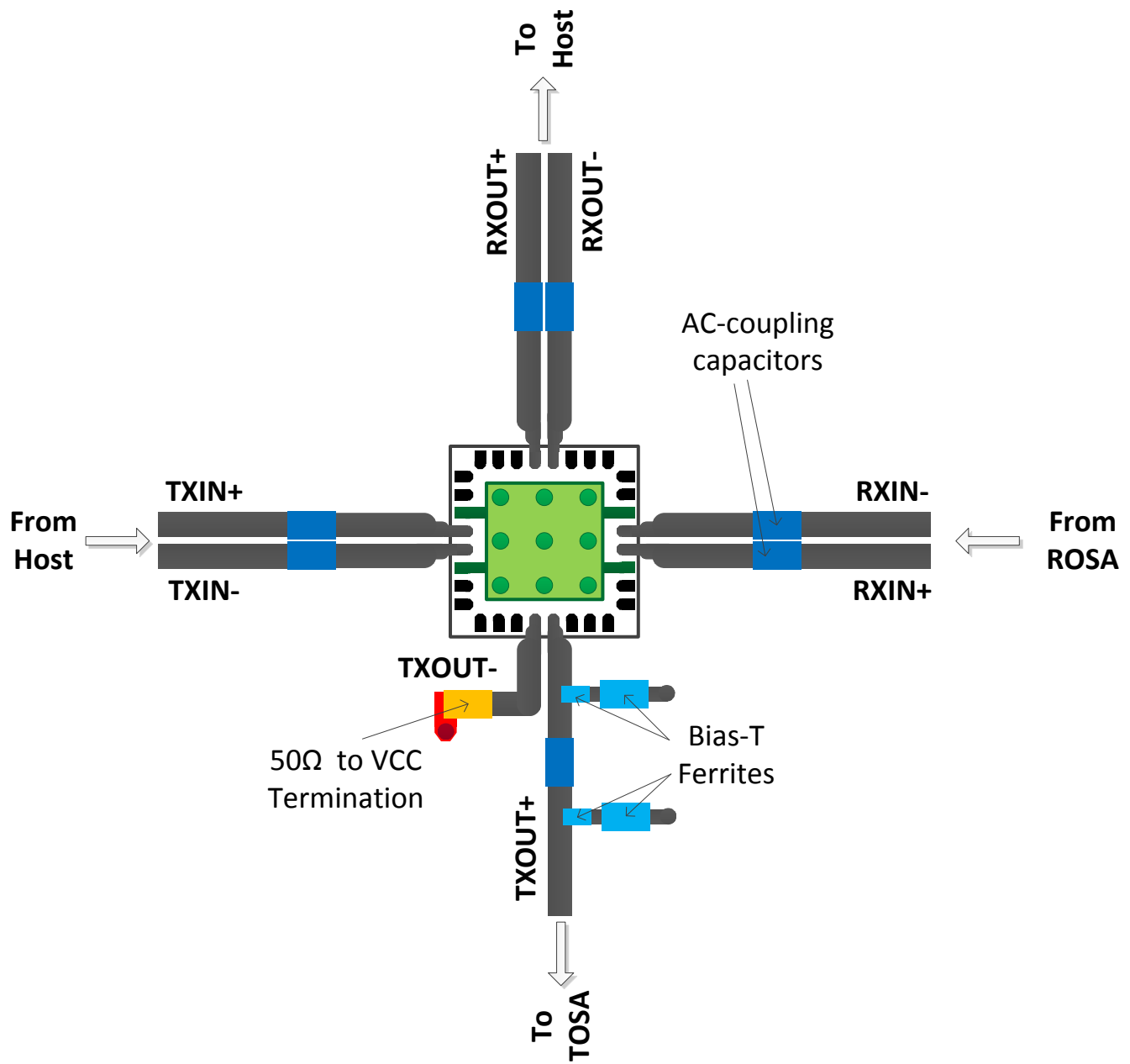
图 73. Board Layout
