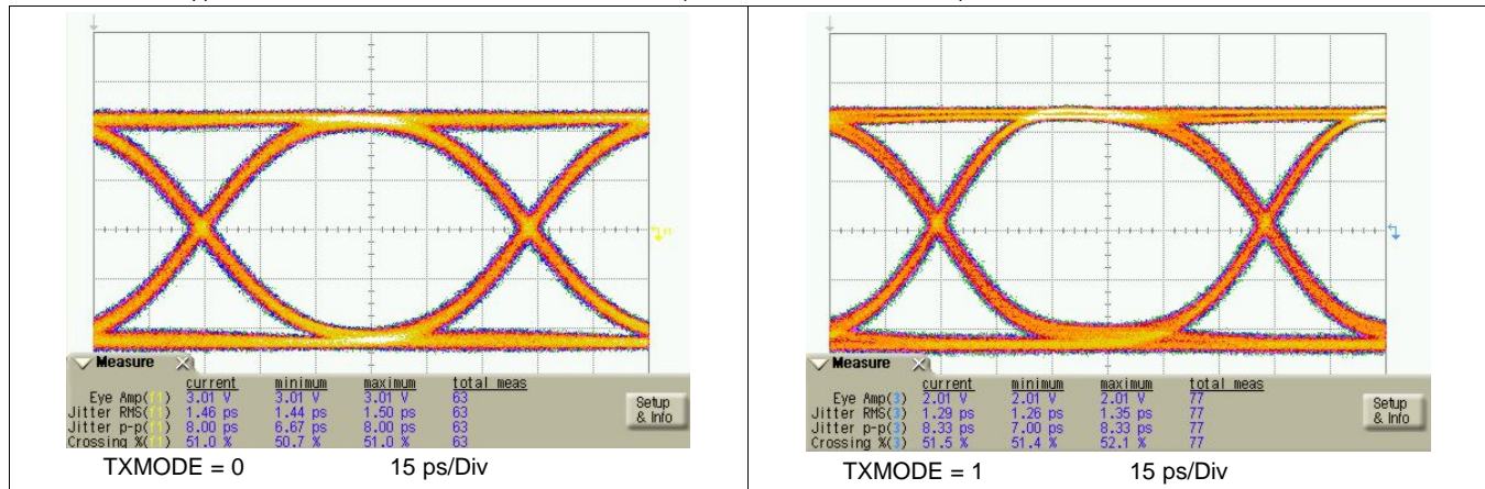
Figure 21. TX Eye-Diagram at 11.3 Gbps
