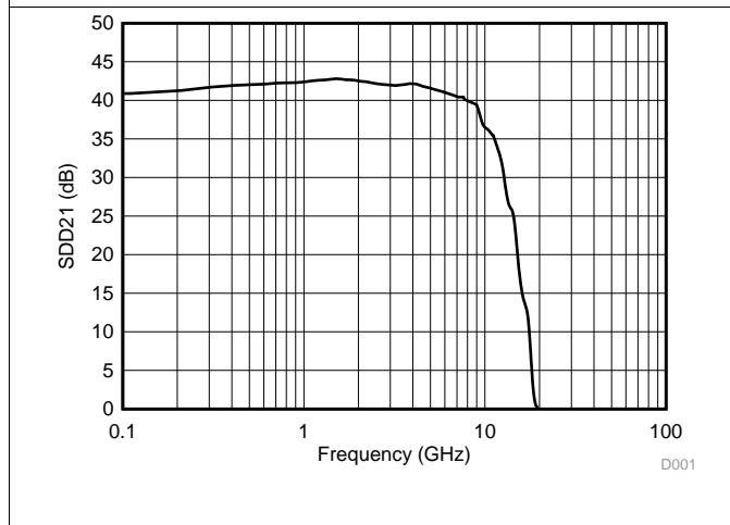
Figure 23. RX Frequency Response (CDR Disabled)
