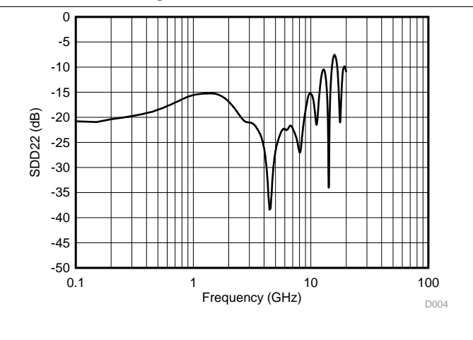
Figure 26. RX Differential Output Return Gain vs Frequency
