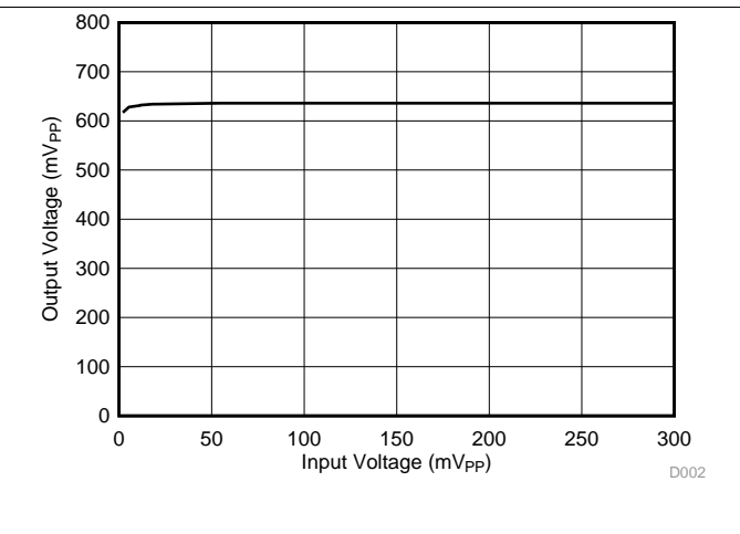
Figure 24. RX Transfer Function
