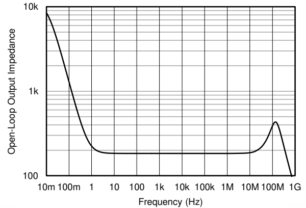
图 26. Open-Loop Output Impedance vs Frequency
