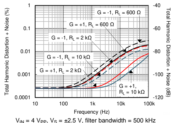
图 30. THD+N vs Frequency
