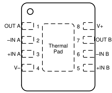
图 5-3. OPA2387: DSG (8-Pin WSON With Exposed Thermal Pad) Package, Top View
