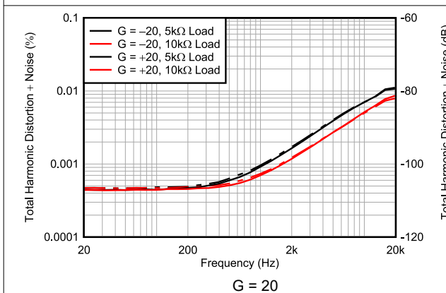
图 6-47. THD+N Ratio vs Frequency
