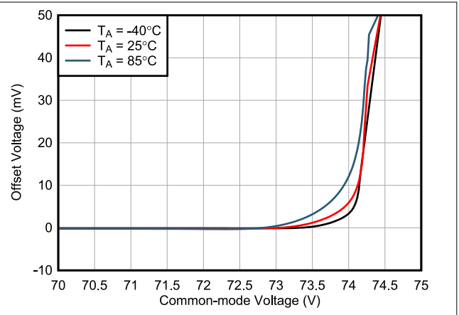
图 6-8. Offset Voltage vs Common-Mode Voltage (High V_{CM} )
