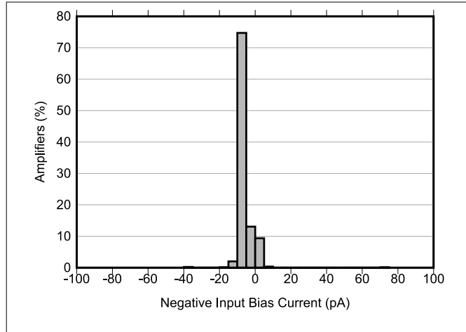
图 6-19. Input Bias Current Production Distribution at 25°C
