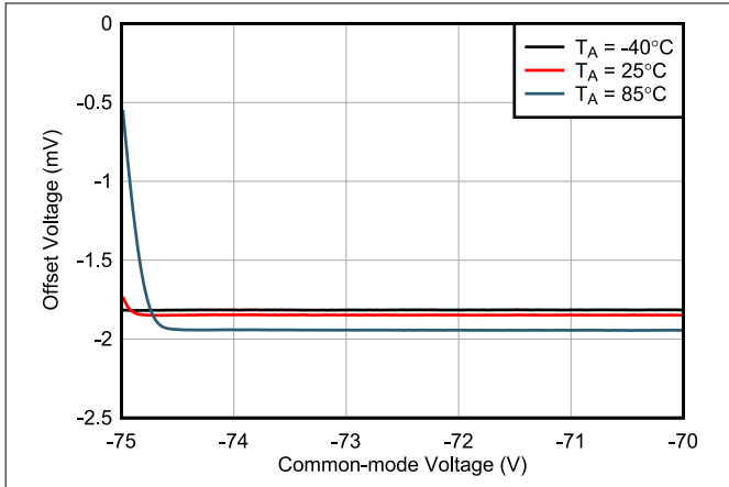
图 6-7. Offset Voltage vs Common-Mode Voltage (Low V_{CM} )
