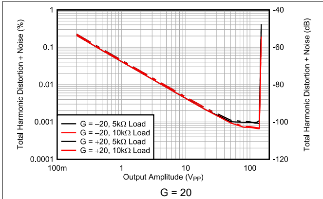
图 6-49. THD+N Ratio vs Output Amplitude
