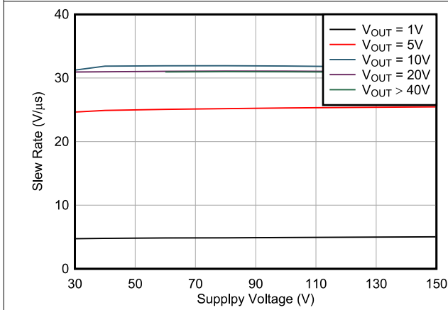
图 6-45. Slew Rate vs Supply Voltage (Noninverting)
