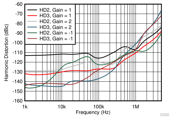
See 图 9-1 and 图 9-2, R_F = 0 \Omega
