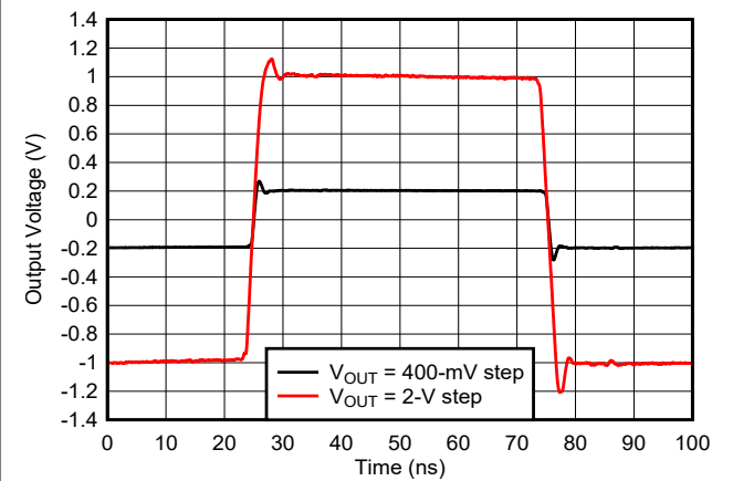
Figure 6-10. Noninverting Large-Signal Pulse Response
