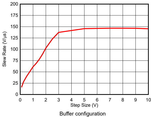
Figure 6-39. Slew Rate vs Output Step Size
