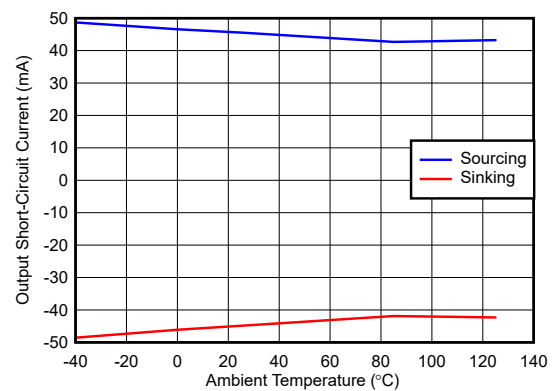
图 7-18. Output Short-Circuit Current vs Ambient Temperature
