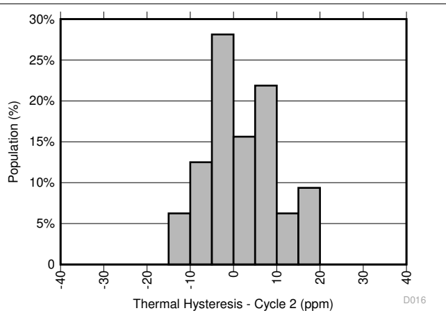
图 7-18. Thermal Hysteresis Distribution (Cycle 2)
