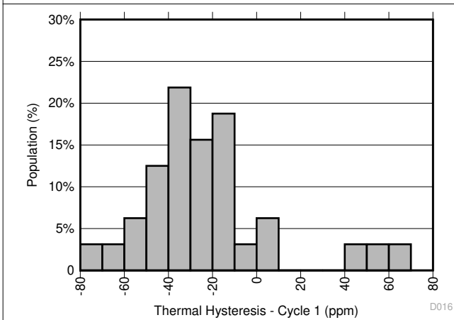
图 7-17. Thermal Hysteresis Distribution (Cycle 1)
