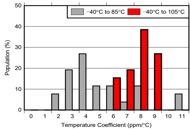
Figure 7-2. Temperature Coefficient Distribution ( V_{REF} = 1.25\text{ V} )
