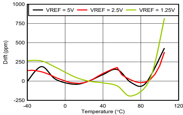
Figure 7-1. Output Voltage Drift vs Free-Air Temperature
