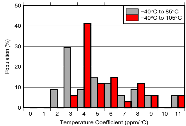
Figure 7-4. Temperature Coefficient Distribution ( V_{REF} = 5.0\text{ V} )
