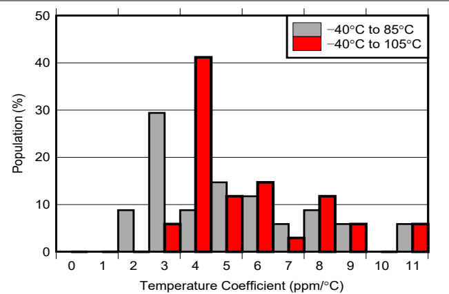
Figure 7-4. Temperature Coefficient Distribution ( V_{REF} = 5.0\text{ V} )
