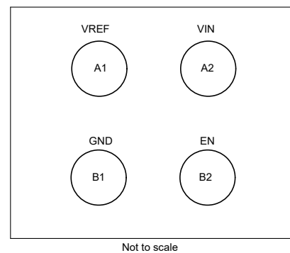
Not to scale Figure 6-2. YBH Package 4-Pin WCSP Top View
