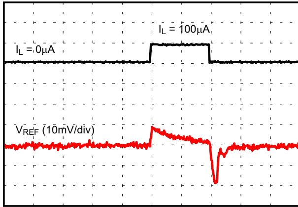
Figure 9-3. Load Transient Response 0 \mu A to 100 \mu A, C_L = 1 \mu F
