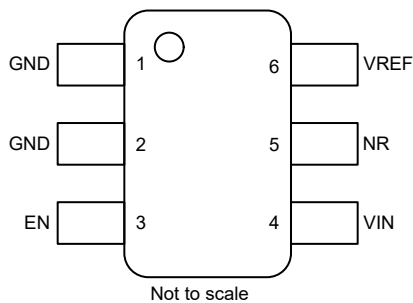
Not to scale Figure 6-1. DBV Package 6-Pin SOT-23 Top View
