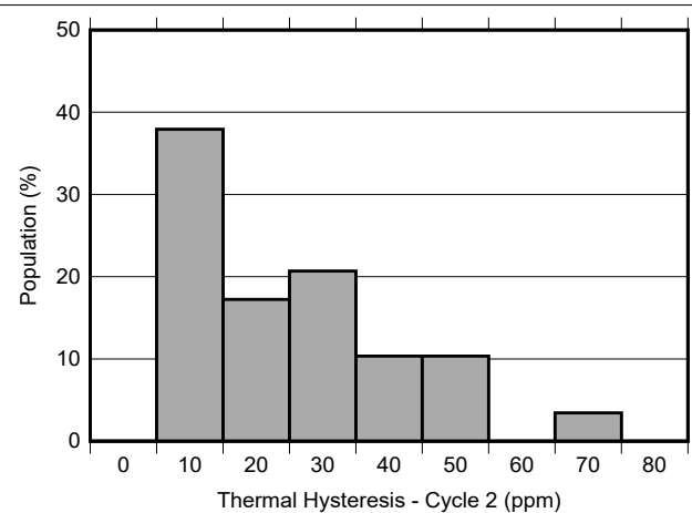
Figure 8-9. Thermal Hysteresis Distribution –40°C to 105°C, Cycle 2
