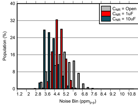
Figure 7-9. 0.1 Hz to 10 Hz Noise Distribution ( V_{REF} = 2.5\text{ V} , C_L = 1\ \mu\text{F} , I_L = 0\text{ mA} )
