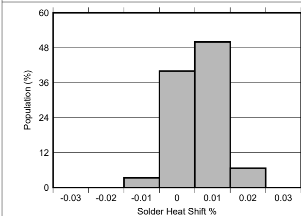
Figure 7-29. Solder Heat Shift Distribution
