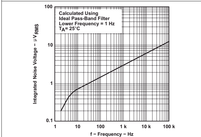
图 6-53. Integrated Noise Voltage vs Frequency
