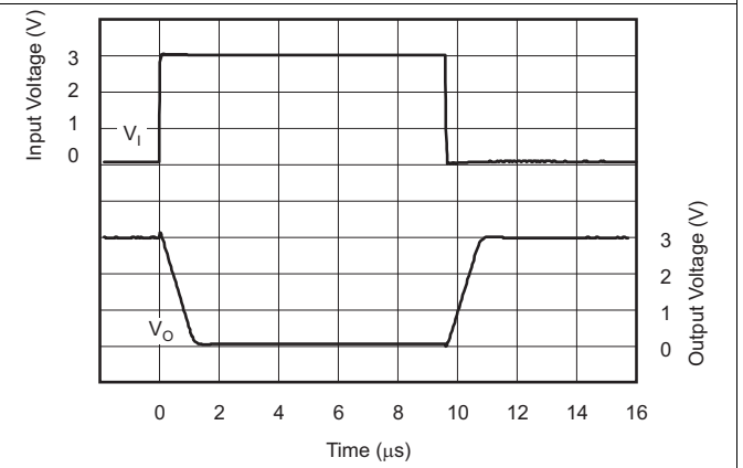
Figure 24. Inverting Large-Signal Response
