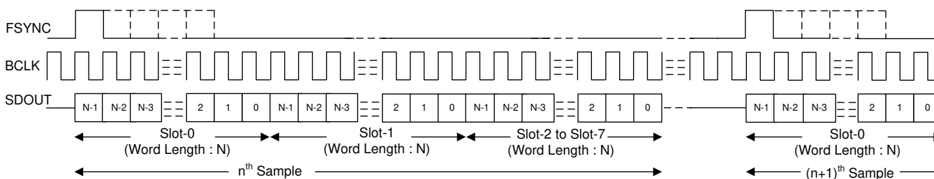
图 23. TDM Mode Standard Protocol Timing (TX_OFFSET = 0)
