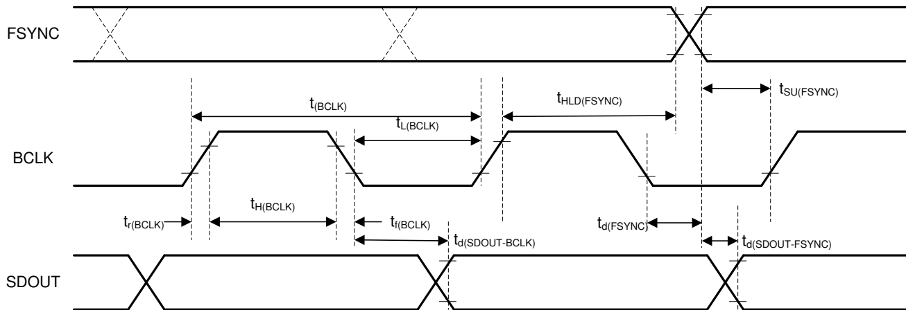
图 3. TDM (With BCLK_POL = 1), I 2 S, and LJ Interface Timing Diagram
