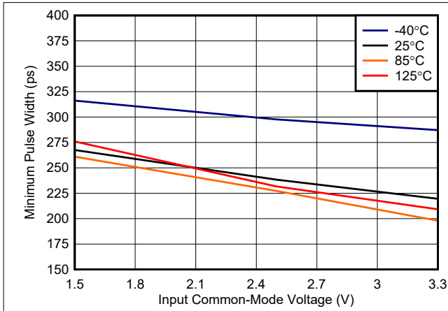
图 6-21. Minimum Pulse Width vs. Common-Mode, 3.3 V
