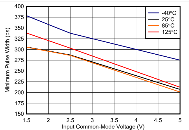
图 6-22. Minimum Pulse Width vs. Common-Mode, 5 V
