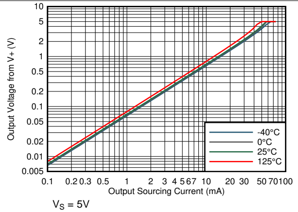
图 28. Output Voltage vs Output Sourcing Current
