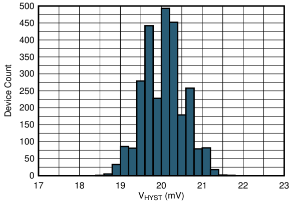
图 39. V HYST Histogram (TLV40x1R2, V S =5V)
