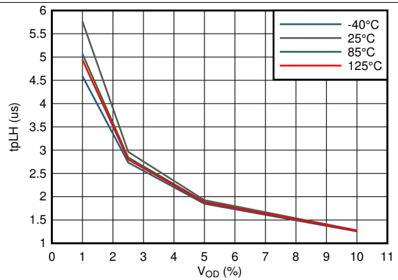
图 30. Propagation Delay Low-High vs Input Overdrive
