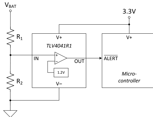
图 45. Under-Voltage Detection
