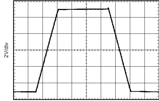
Time (4µs/div) G = -1, R_L = 10k\Omega , C_L = 100pF
