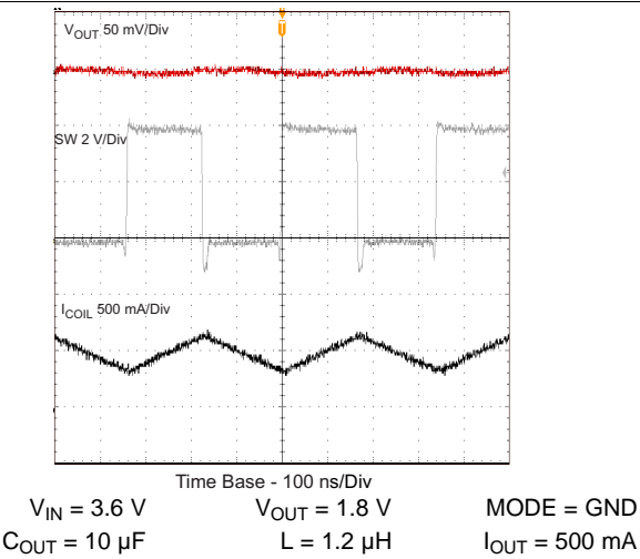
Figure 13. Typical Operation (PWM Mode)
