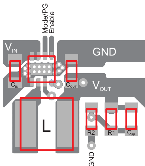
Figure 24. PCB Layout
