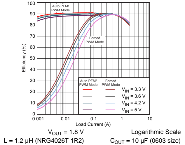
Figure 4. Efficiency vs Load Current Auto PFM and PWM Mode vs. Forced PWM Mode
