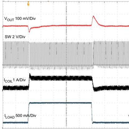
Figure 15. Load Transient Response, MODE = V_{IN} PWM Mode 0.2 A To 1 A
