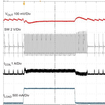
Figure 16. Load Transient PFM Mode 20 mA to 250 mA
