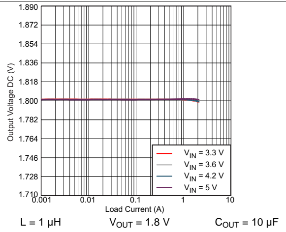
Figure 6. Output Voltage Accuracy vs Load Current Forced PWM MODE
