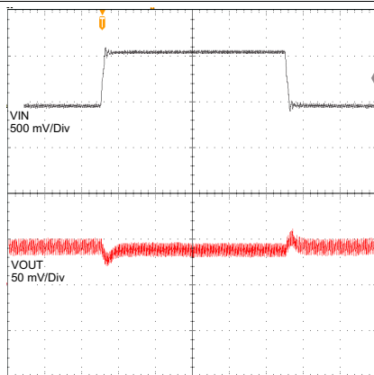
Figure 17. Load Transient Response 200 mA To 1500 mA
