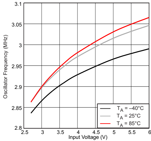
Figure 9. Oscillator Frequency vs Input Voltage
