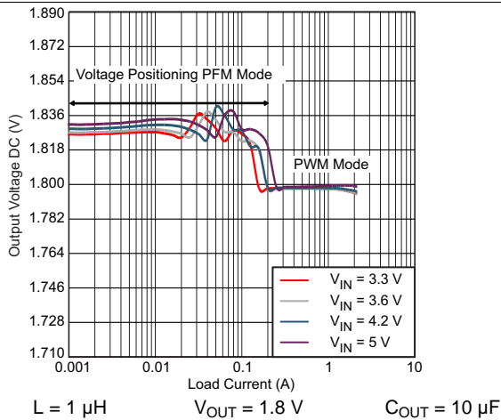
Figure 5. Output Voltage Accuracy vs Load Current Auto PFM and PWM MODE
