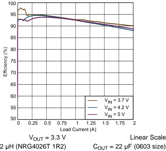
Figure 3. Efficiency vs Load Current Auto PFM and PWM MODE
