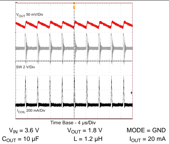
Figure 14. Typical Operation (PFM Mode)
