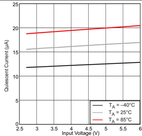
Figure 8. Quiescent Current vs Input Voltage and Ambient Temperature
