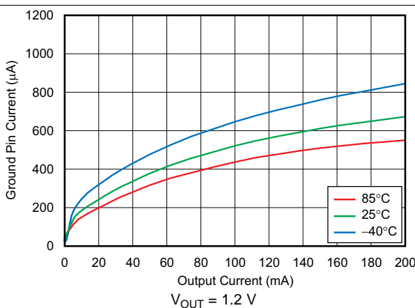
Figure 23. Ground Pin Current vs Output Current
