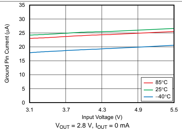
Figure 18. Ground Pin Current vs Input Voltage
