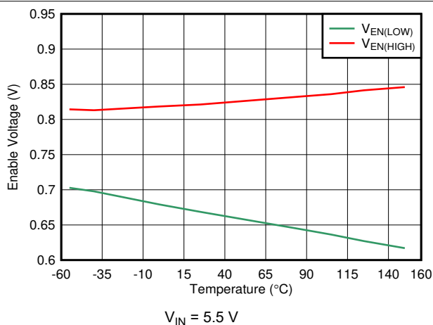
图 6-12. EN High and Low Threshold vs Temperature
