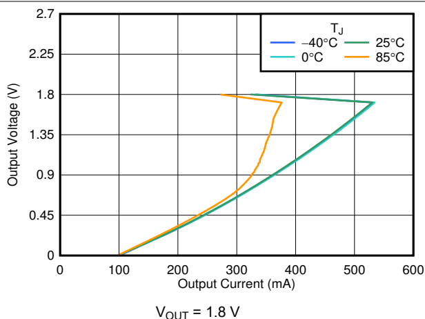
图 6-8. Foldback Current Limit vs I_{OUT}
