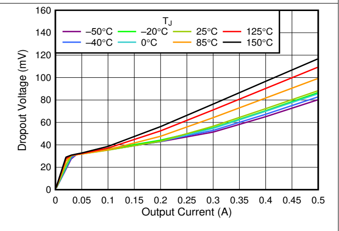
图 6. 5.5-V Dropout Voltage vs I_{OUT}
