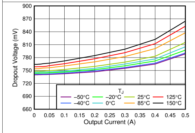
图 5. 0.55-V Dropout Voltage vs I_{OUT}
