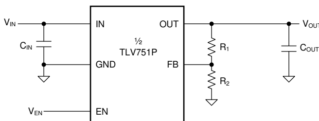
图 38. Adjustable Operation
