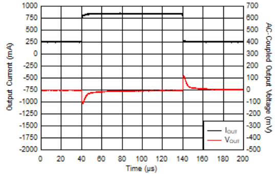
Figure 6-8. I_{OUT} Transient From 250 mA to 850 mA
