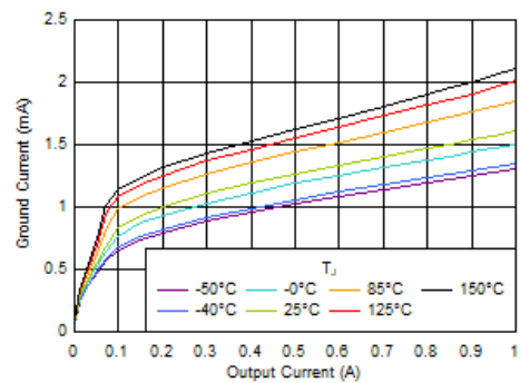
Figure 6-5. I_{GND} vs I_{OUT}
