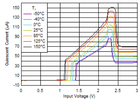
Figure 6-4. I_Q Increase Below Minimum V_{IN}
