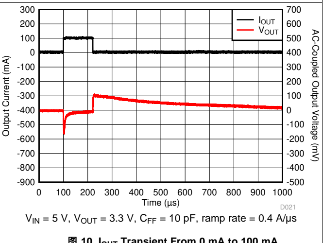
图 10. I_{OUT} Transient From 0 mA to 100 mA
