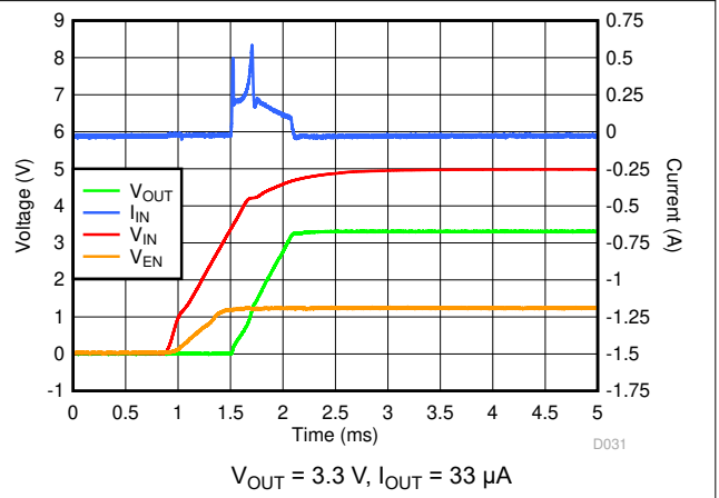
图 7-34. Startup Inrush Current With C_{OUT} = 47\text{ }\mu\text{F}
