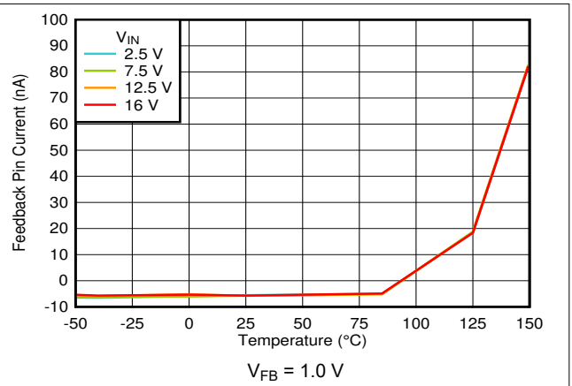
图 7-32. I_{FB} vs Temperature
