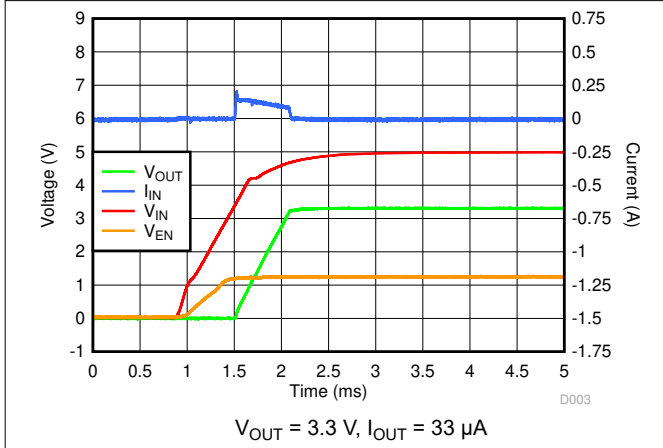
图 7-33. Startup Inrush Current With C_{OUT} = 22\text{ }\mu\text{F}
