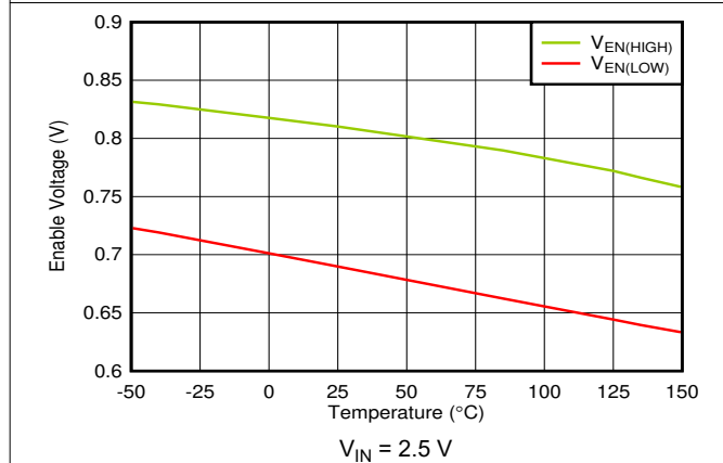
图 7-23. V_{EN} Thresholds vs Temperature
