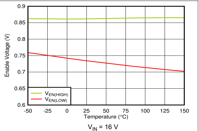
图 7-24. V_{EN} Thresholds vs Temperature
