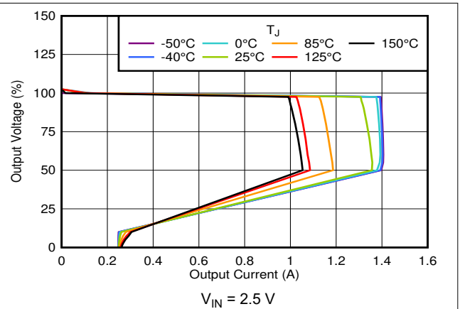
图 7-20. Foldback Current Limit vs Temperature
