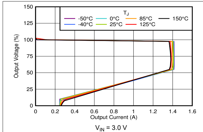
图 7-19. Foldback Current Limit vs Temperature
