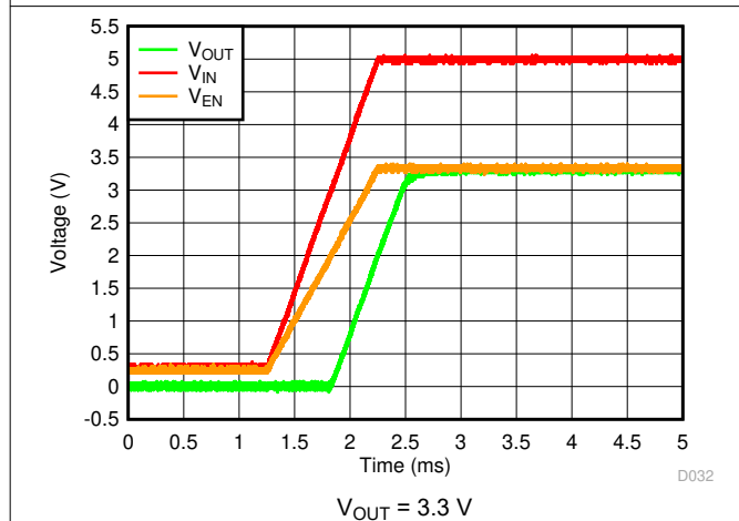
图 7-21. Startup With Separate V_{EN} and V_{IN}
