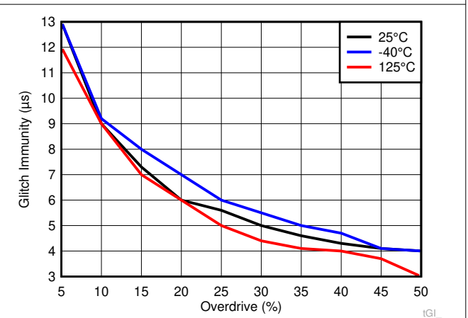
图 7-26. Glitch Immunity Versus Overdrive for TLV803EA29
