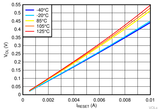
图 7-12. Low Voltage Output Versus Output Current for TLV809EA29, VDD = 1.7 V
