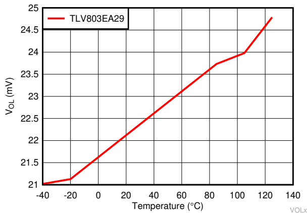
图 7-13. Low Voltage Output Verses Temperature for TLV803EA29, VDD = 1.7 V
