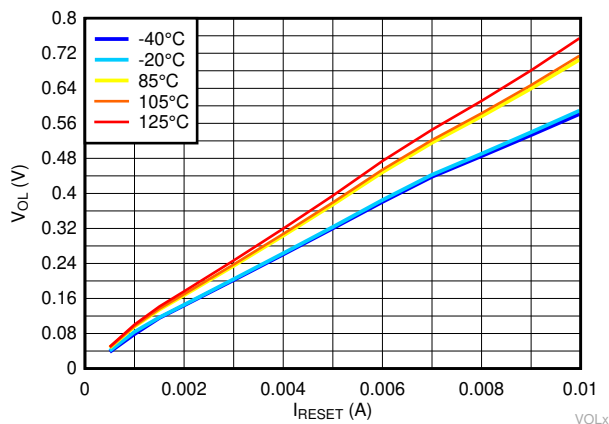
图 7-11. Low Voltage Output Versus Output Current for TLV803EA29, VDD = 1.7 V
