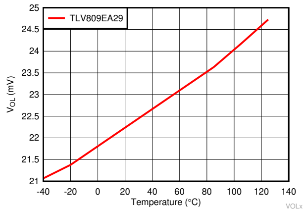
图 7-14. Low Voltage Output Verses Temperature for TLV809EA29, VDD = 1.7 V
