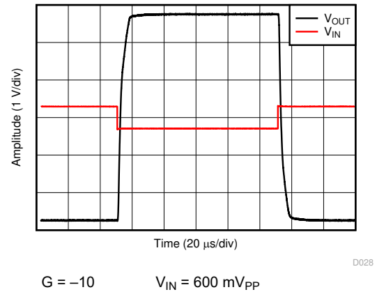
Figure 7-28. Overload Recovery
