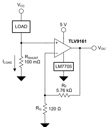
Figure 8-1. TLV9161-Q1 in a Low-Side, Current-Sensing Application
