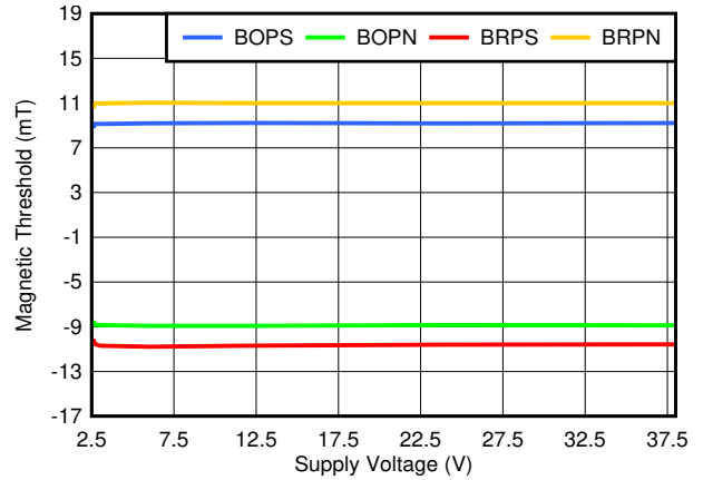
图 7-12. TMAG5123D Magnetic Thresholds vs Voltage
