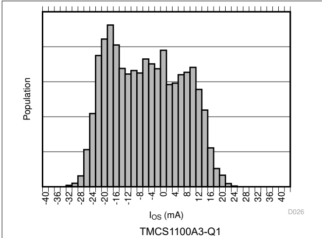
图 7-7. Input Offset Current Production Distribution
