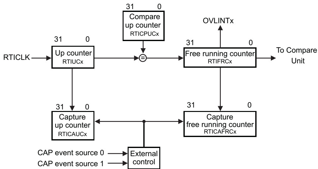
图 6-12. Counter Block Diagram
