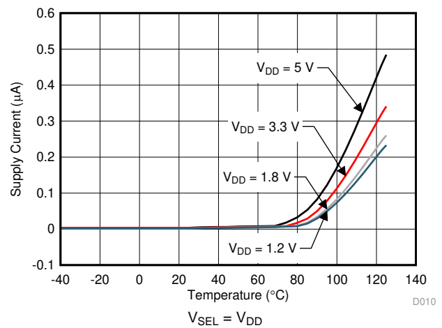
图 10. Supply Current vs Temperature
