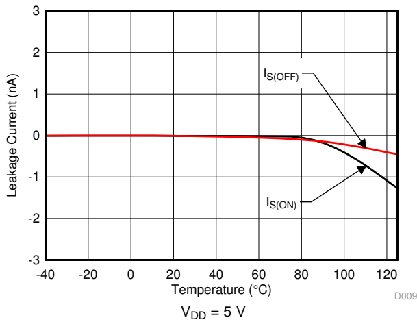
图 9. Leakage Current vs Temperature
