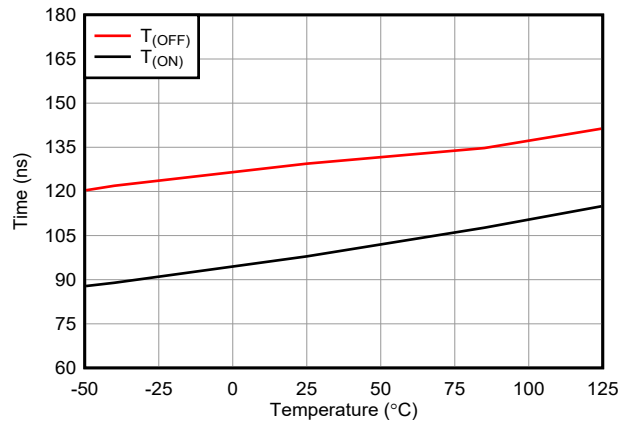
Figure 6-19. T_{ON} (EN) and T_{OFF} (EN) vs Temperature
