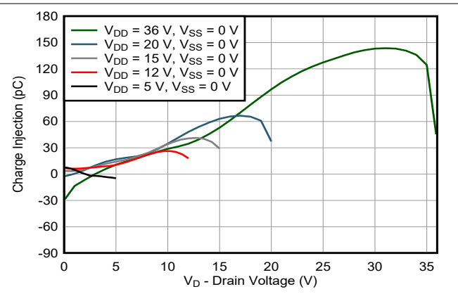
Figure 6-16. Charge Injection vs Drain Voltage – Single Supply
