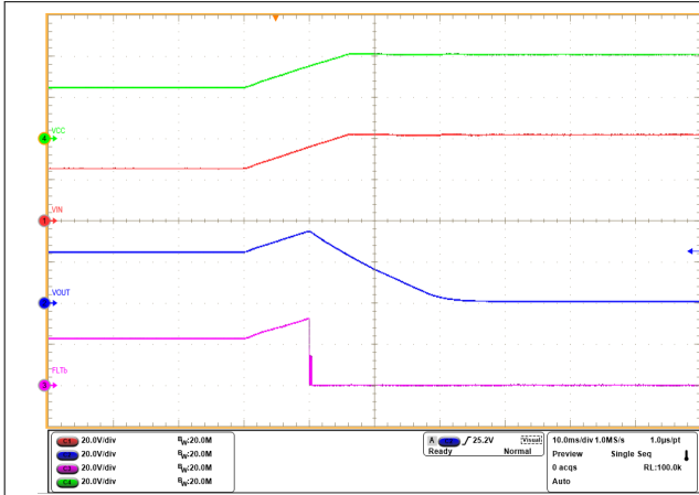
图 9-2. Overvoltage Protection up to 40 V
