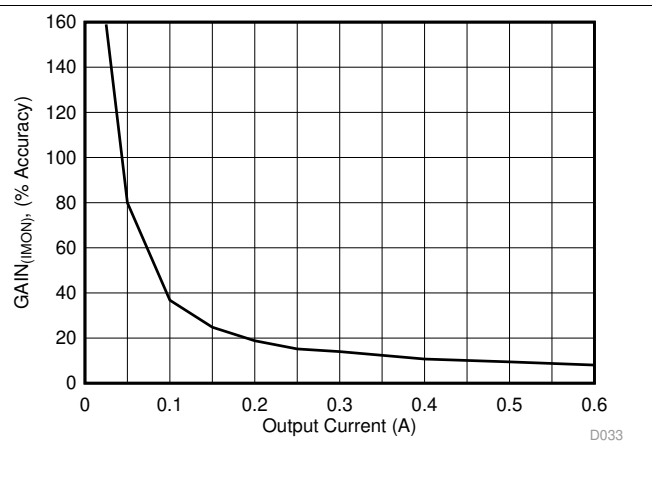
图 10. IMON Gain Accuracy at Low Output Current Levels
