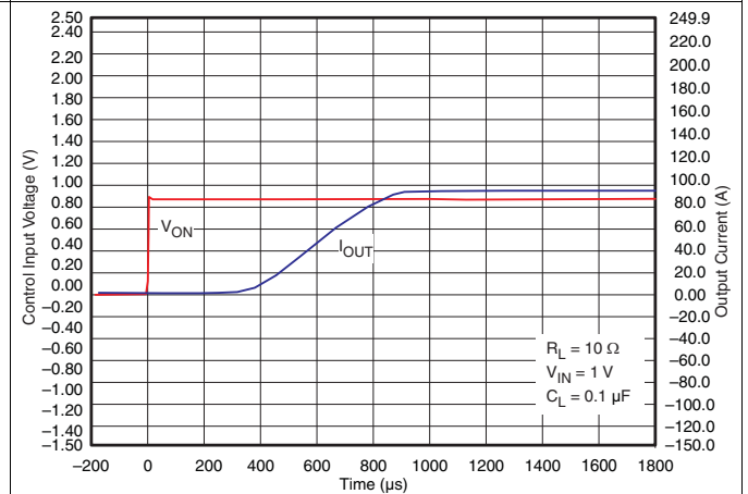
Figure 41. t_{ON} Response
