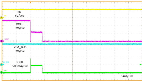
图 11-28. OUT short to 5.1-Ω Load
