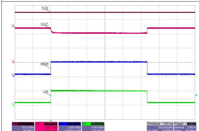
图 10-11. Over Load: Step Change in Load from 12 \Omega to 2 \Omega and Back
