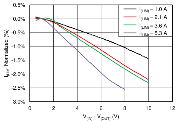
图 7-20. Current Limit Normalized (%) vs V_{(IN)} - V_{(OUT)}
