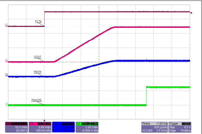
图 10-16. Power Good Response During Turn-ON
