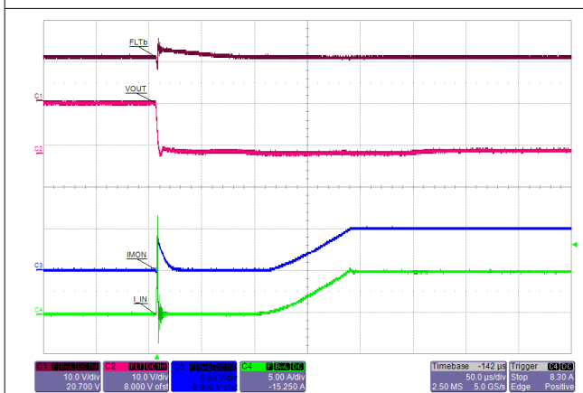
图 10-13. Hot Short: Fast Trip and Current Regulation
